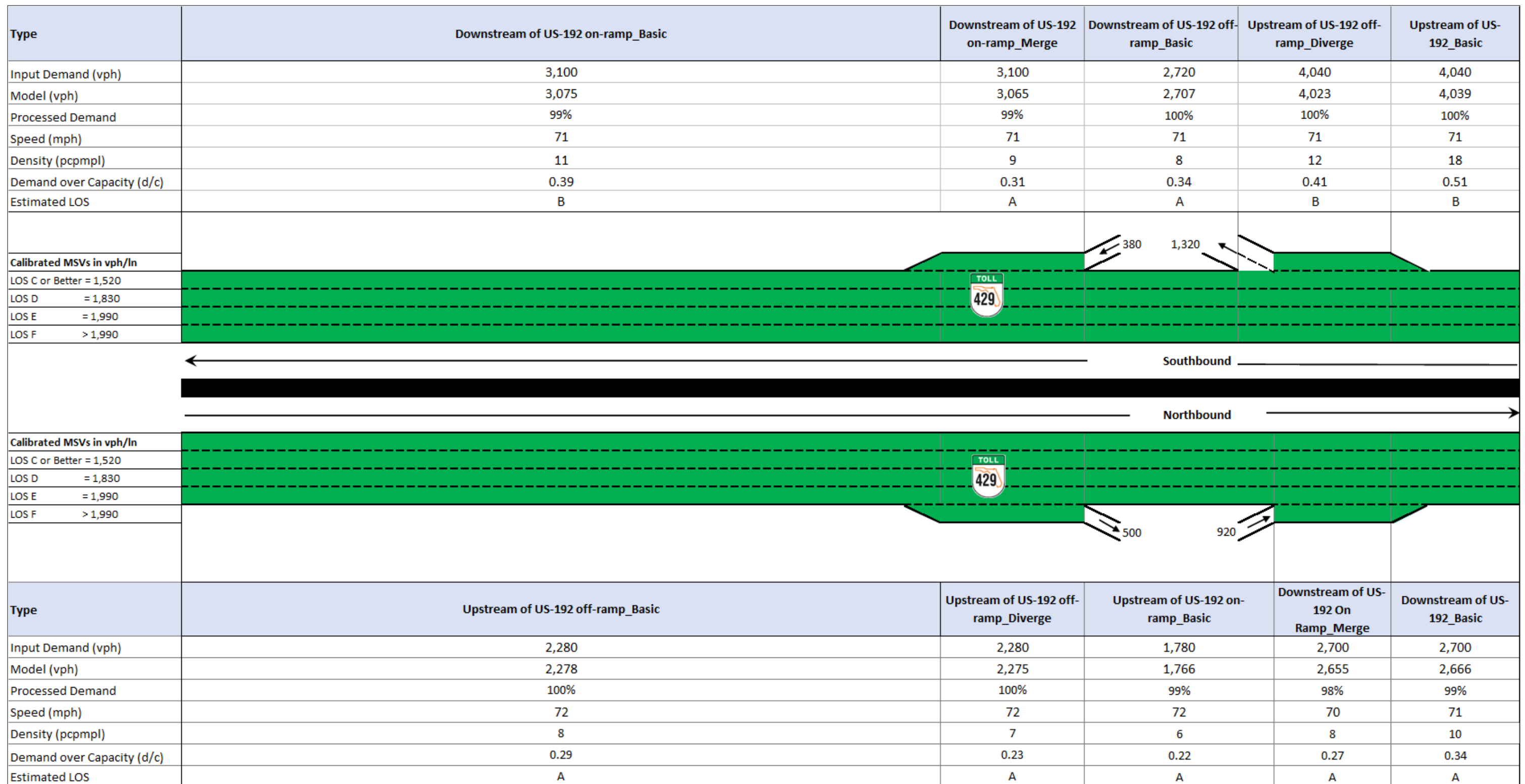
Figure 6.7 2030 PM Build w/o Livingston Road Interchange Design Hour Vissim Freeway Performance Results
