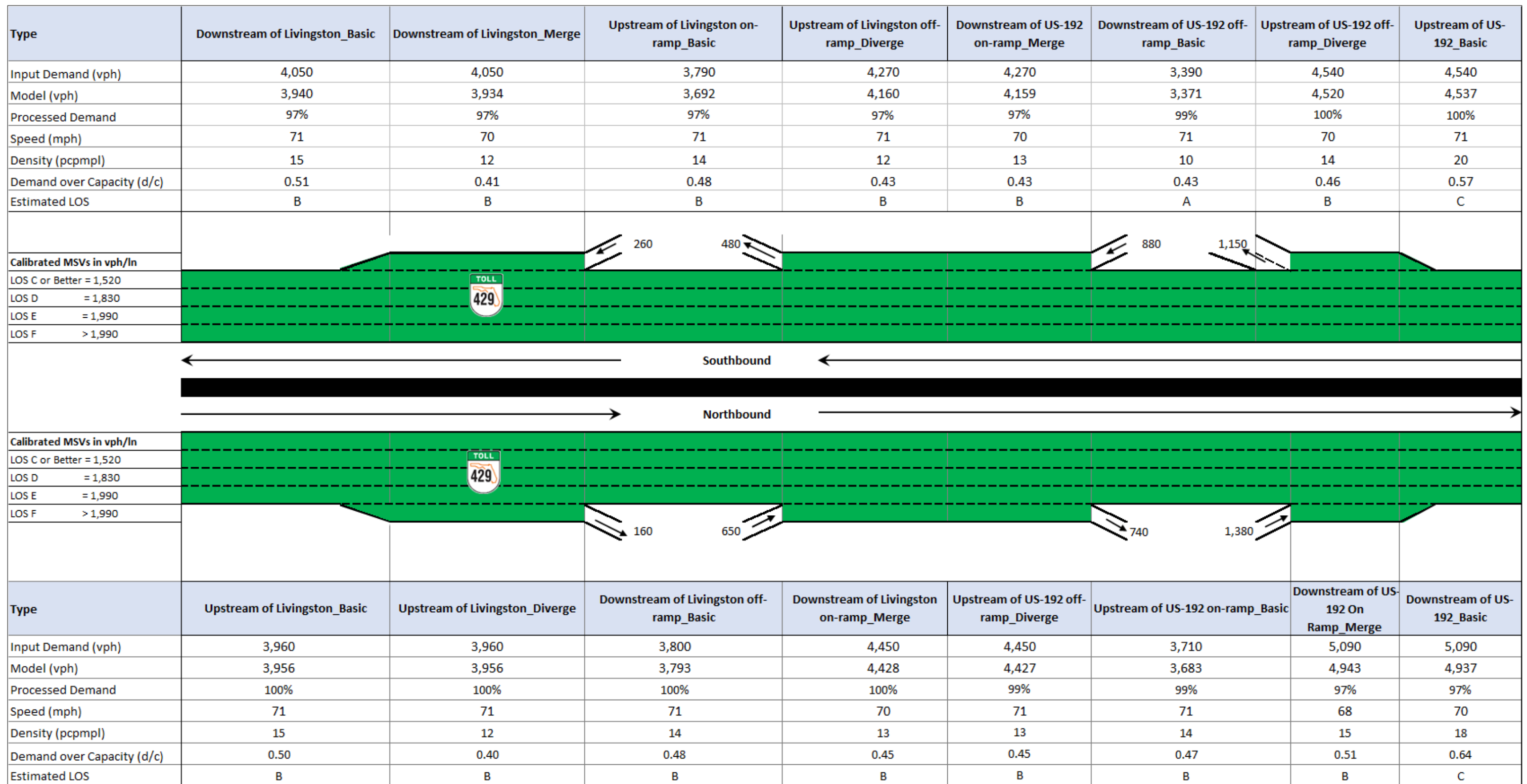
Figure 6.15 2050 AM Build w/Livingston Road Interchange Design Hour VISSIM Freeway Performance Results
