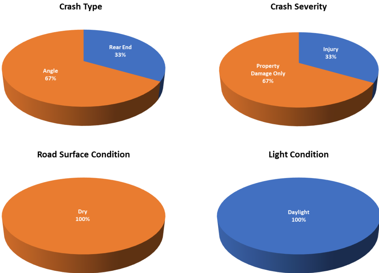
Figure 3.22 Seidel Road and SR 429 Intersections Crash Data Summary (2014-2018)
