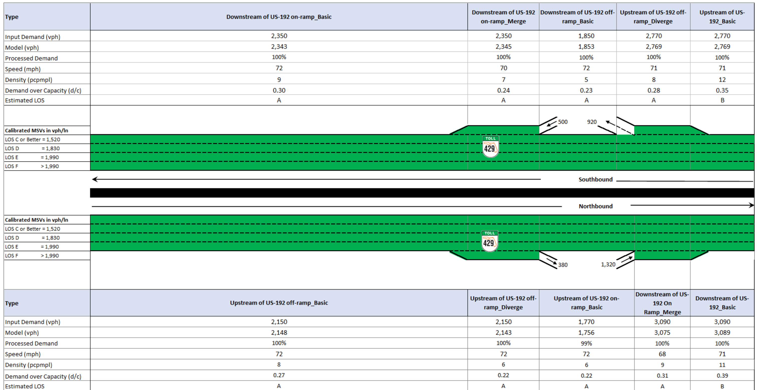
Figure 6.6 2030 AM Build w/o Livingston Road Interchange Design Hour Vissim Freeway Performance Results
