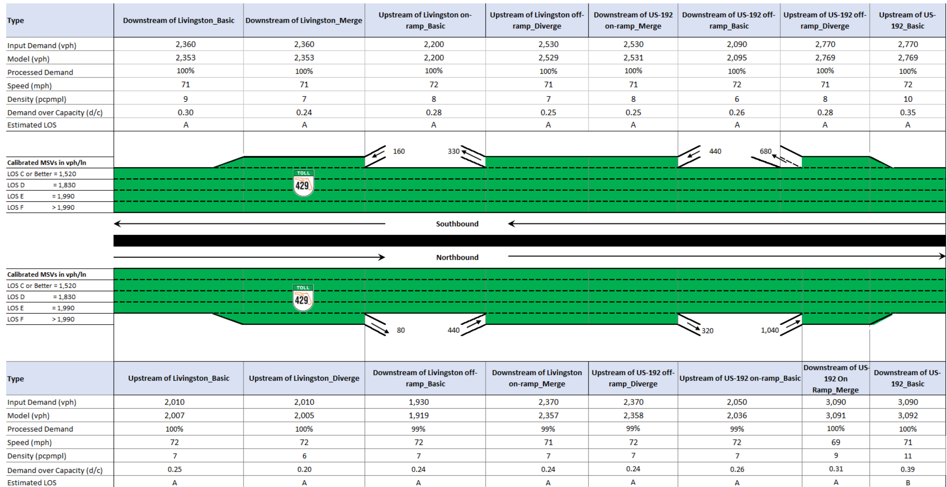
Figure 6.8 2030 AM Build w/Livingston Road Interchange Design Hour Vissim Freeway Performance Results
