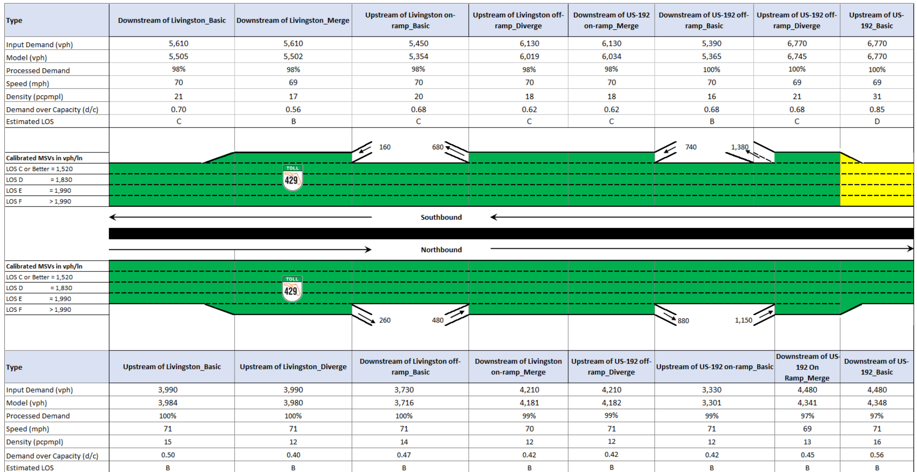
Figure 6.16 2050 PM Build w/Livingston Road Interchange Design Hour VISSIM Freeway Performance Results
